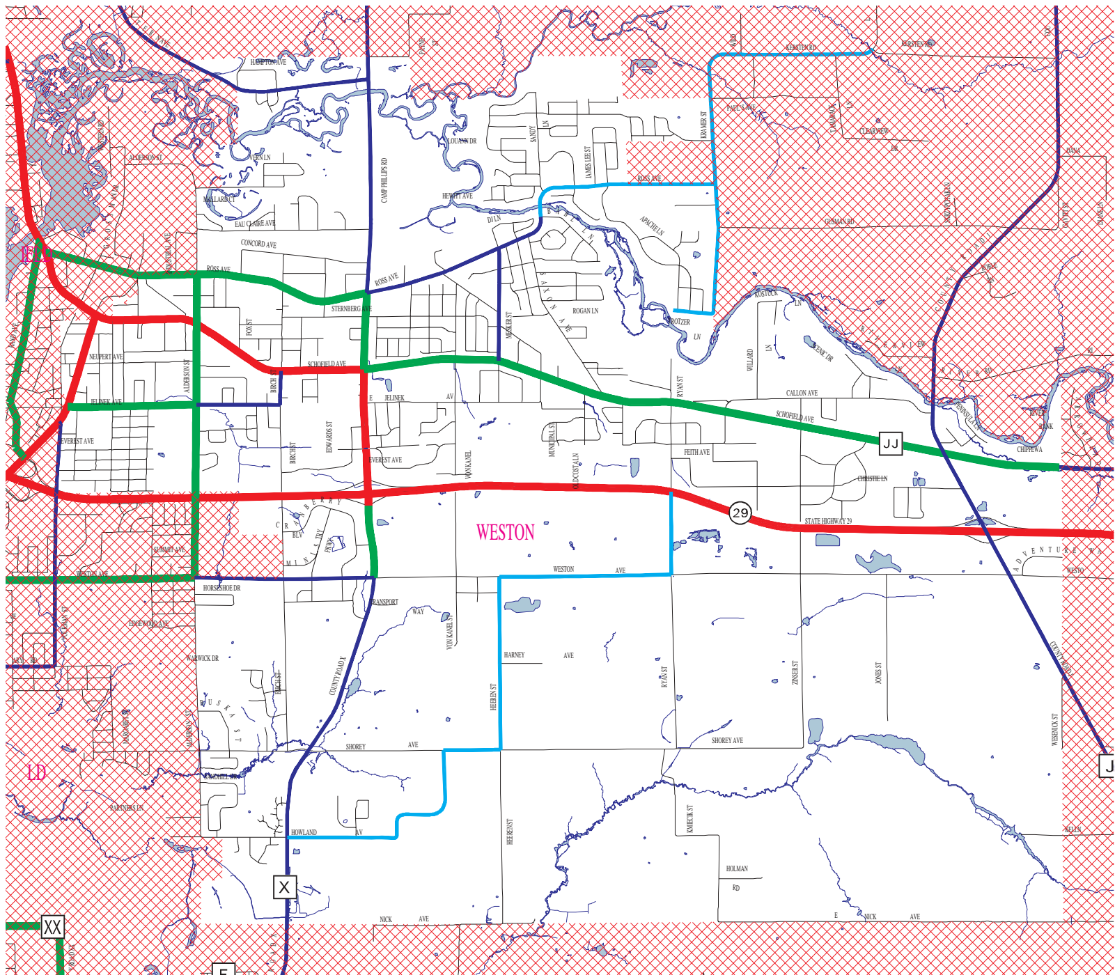
Figure 4-1 Functional Classification of Roads V-WESTON
