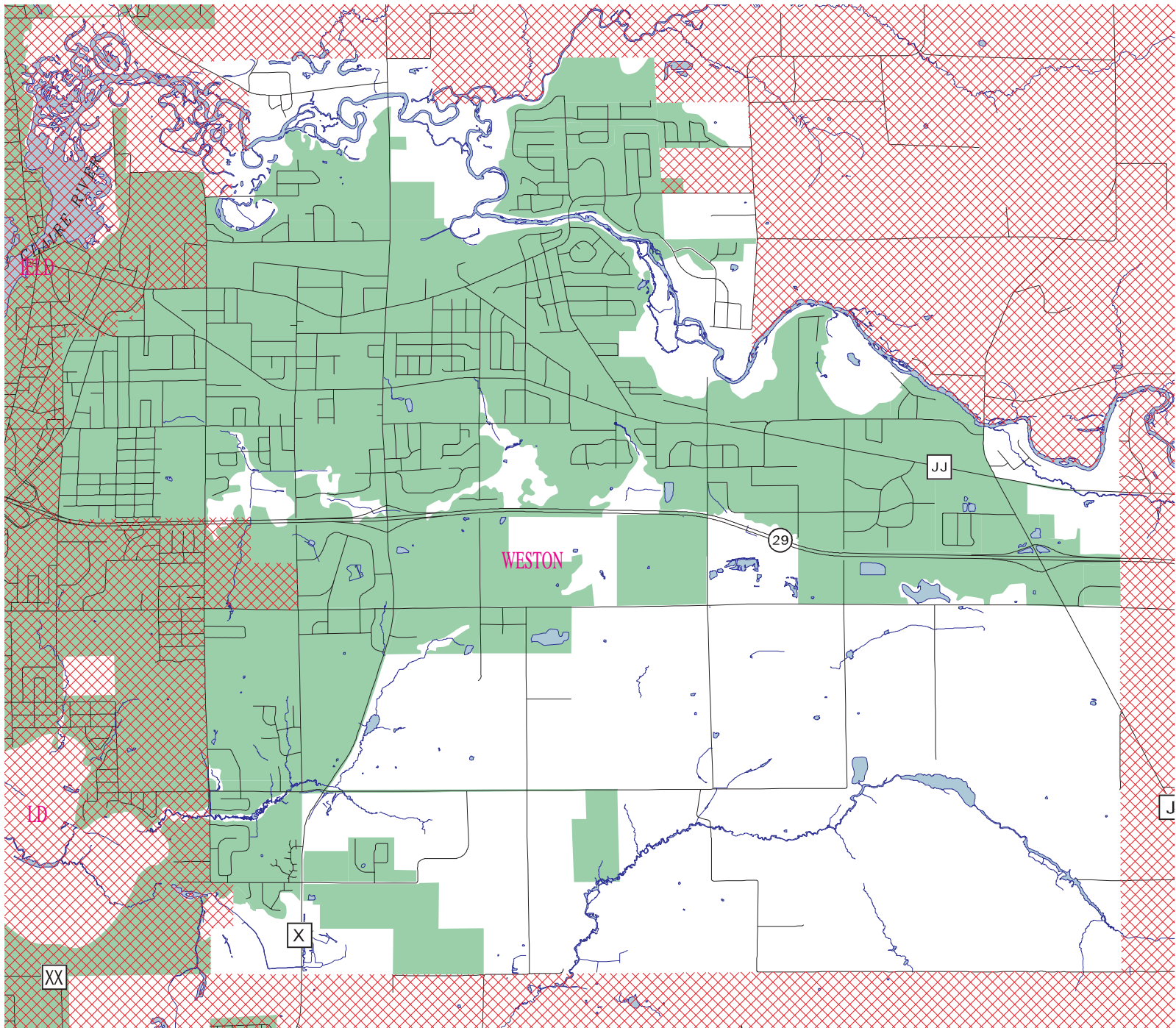
Figure 6-1 Sewer Service Areas V-WESTON
