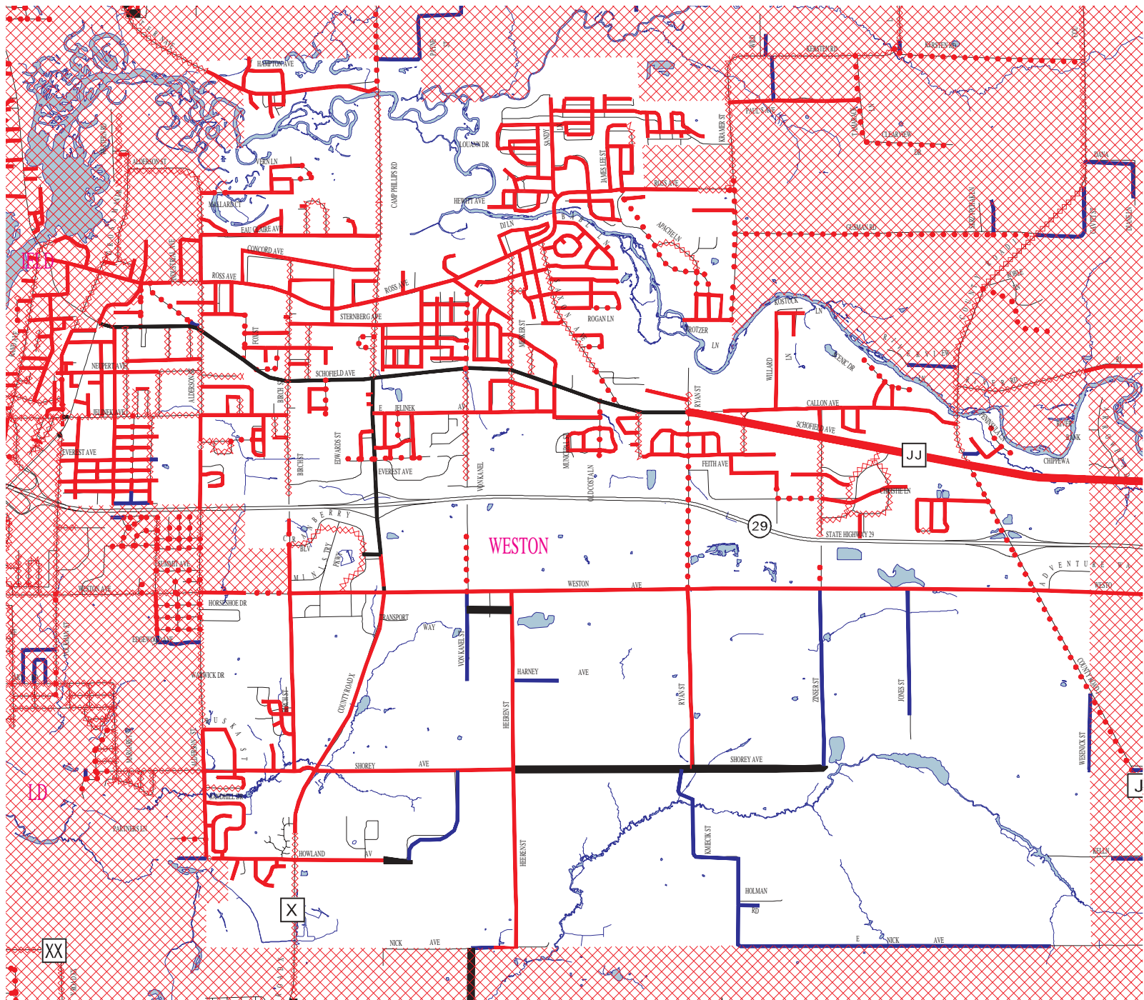
Figure 4-4 Road Surface Types V-WESTON
